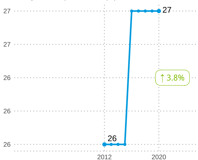
Annual mean concentrations of fine particulate matter (PM2.5) in urban areas ( \mu\text{g}/\text{m}^3 )
